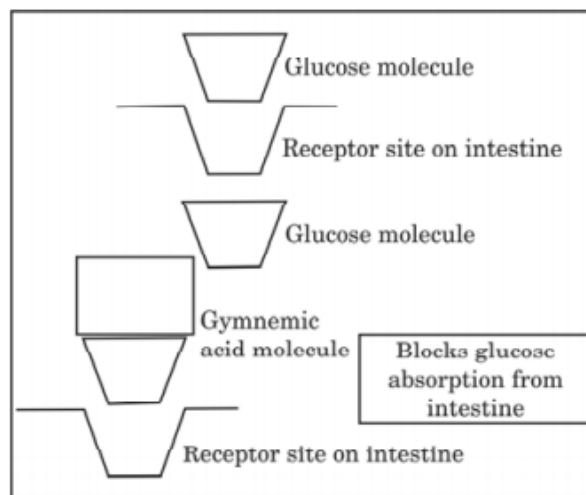
Figure 3: Gymnemic acid competes with a gut receptor site (Kanetkar P, et al., 2007)
