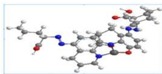
Figure 17: Suggest structural formula of M-complexes
